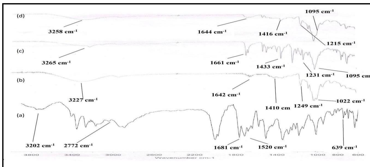
FIGURE 7 FTIR Spectra of (a) LER (b) HPβCD (c) Physical Mixture LER: HPβCD (1:1.5) (d) HPBCDF2
