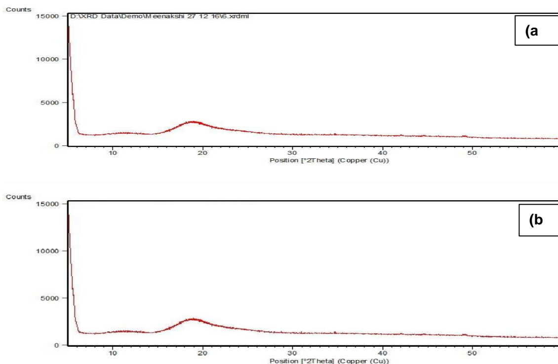
FIGURE 12 Powdered X Ray diffraction patterns of Optimized inclusion complex of LER and HPBCD (a) at zero time (b) after storage of 6 months
