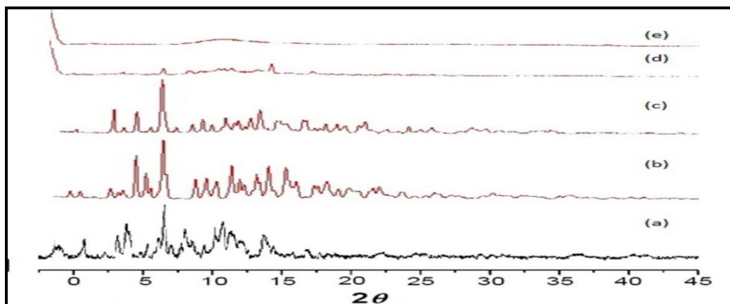
FIGURE 8 XRD Pattern of (a) LER (b) Physical Mixture LER : βCD (1:1.5) (c) BCDF2 (d) Physical Mixture LER : HPβCD (1:1.5) (e) HPBCDF2
