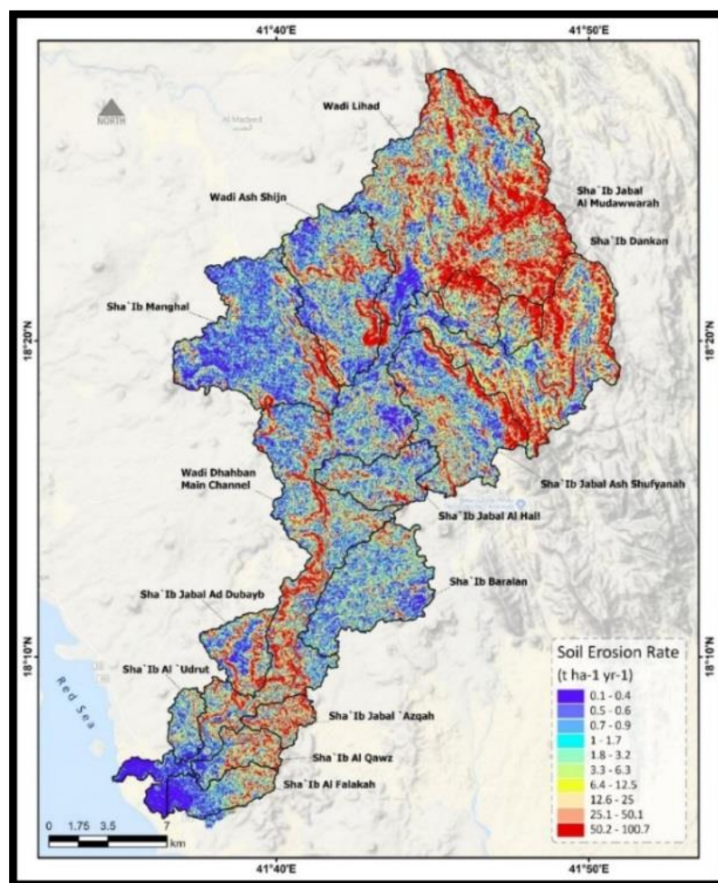
Fig. 16: The annual average soil loss of Wadi Dhahban
