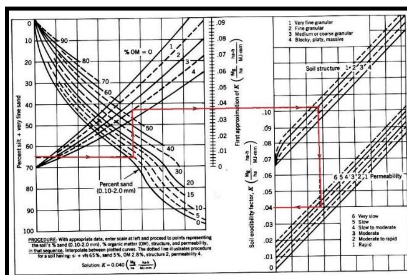
Fig.15: Soil-Erodibility Nomograph in SI units
