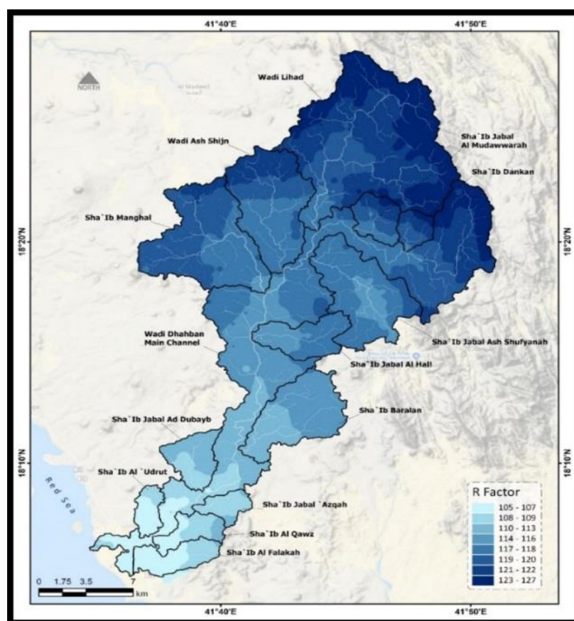
Fig. 6: Factor R of RUSLE equation calculated for Wadi Dhahban
