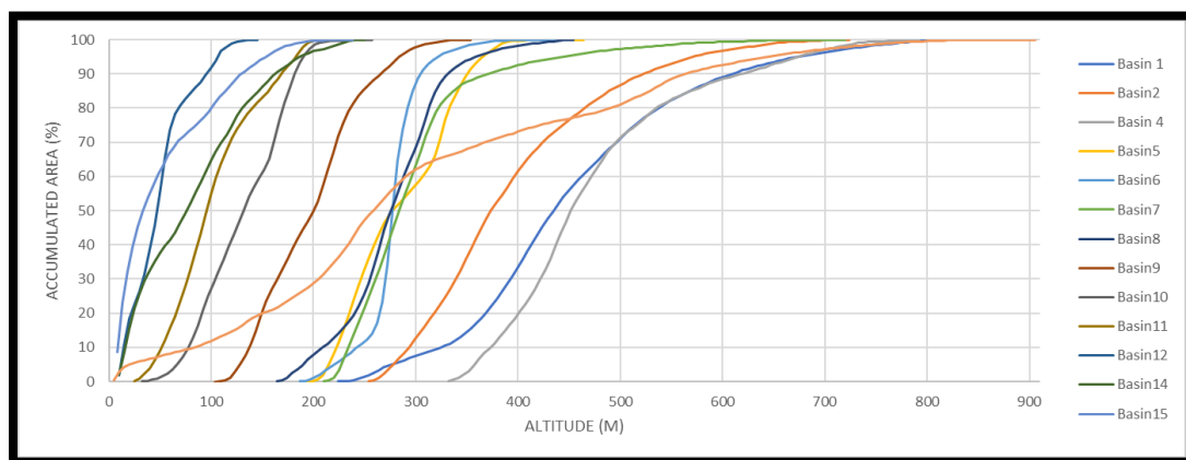
Fig. 5: Classification of the hypsometric curves of the sub-watersheds of Wadi Dhahban
