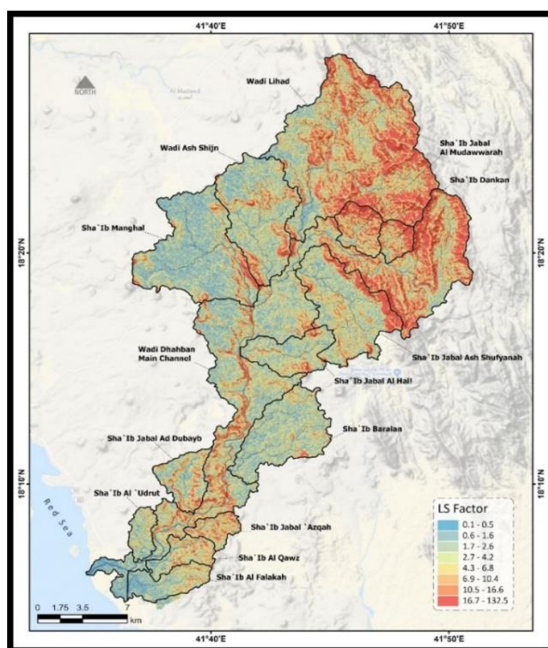
Fig. 11: Factor LS of RUSLE equation calculated for Wadi Dhahban
