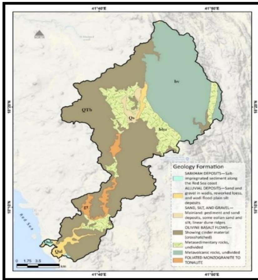
Fig. 2: Geology formation of Wadi Dhahban
