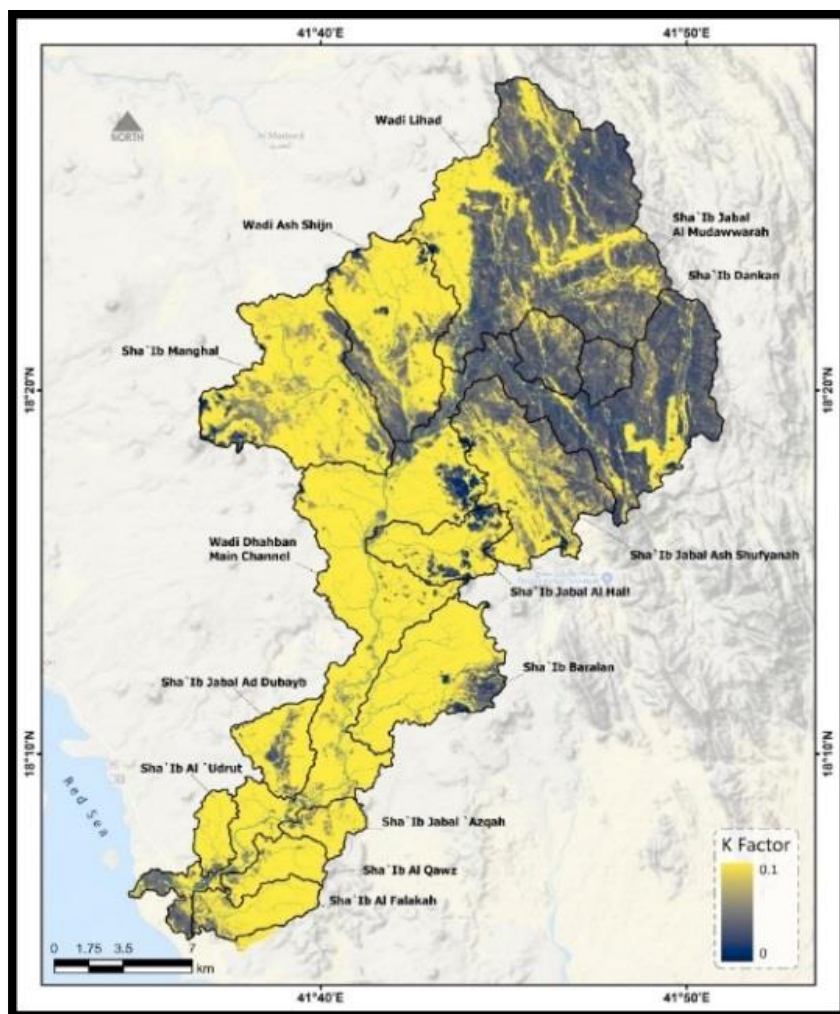
Fig. 7: Factor K of RUSLE equation calculated for Wadi Dhahban
